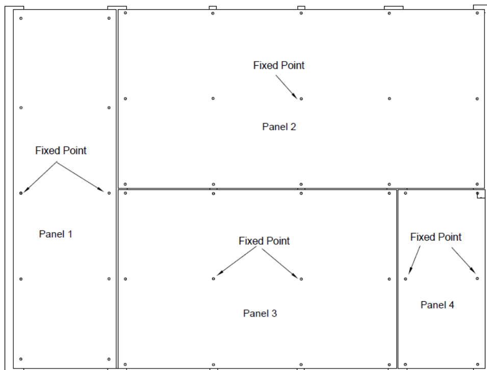
Image 1– Example of cladding with Ceramapanel® A1 fibre-cement panels. In some cases, the geometry of the panel and the facade layout may require two fixed points.
