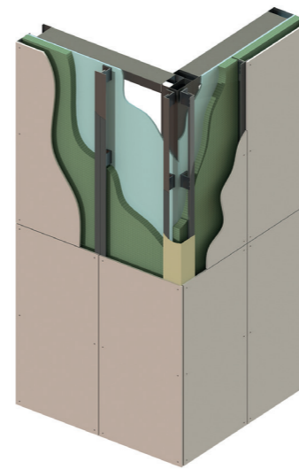
Face-Fix Assembly
