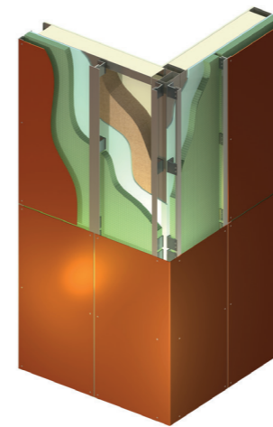
Face-Fix Assembly
